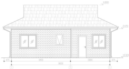
Elevation of A axis 1:100
