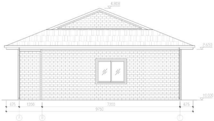
Elevation of 6 axis 1:100
