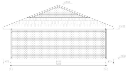
Elevation of 1 axis 1:100
