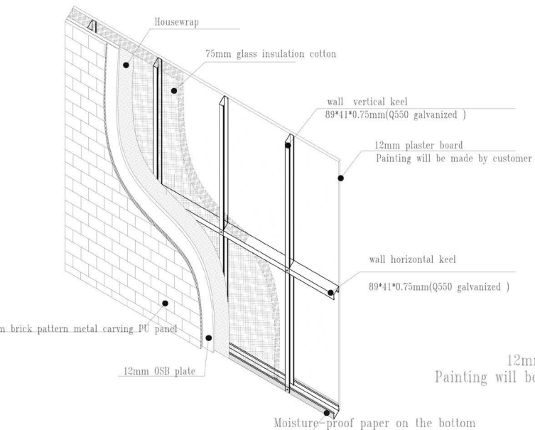
Outside wall details
