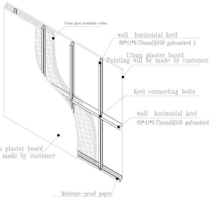
Inside wall details
